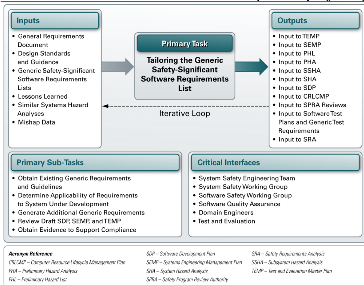
Figure 4-29: Tailoring the Generic Safety Requirements
